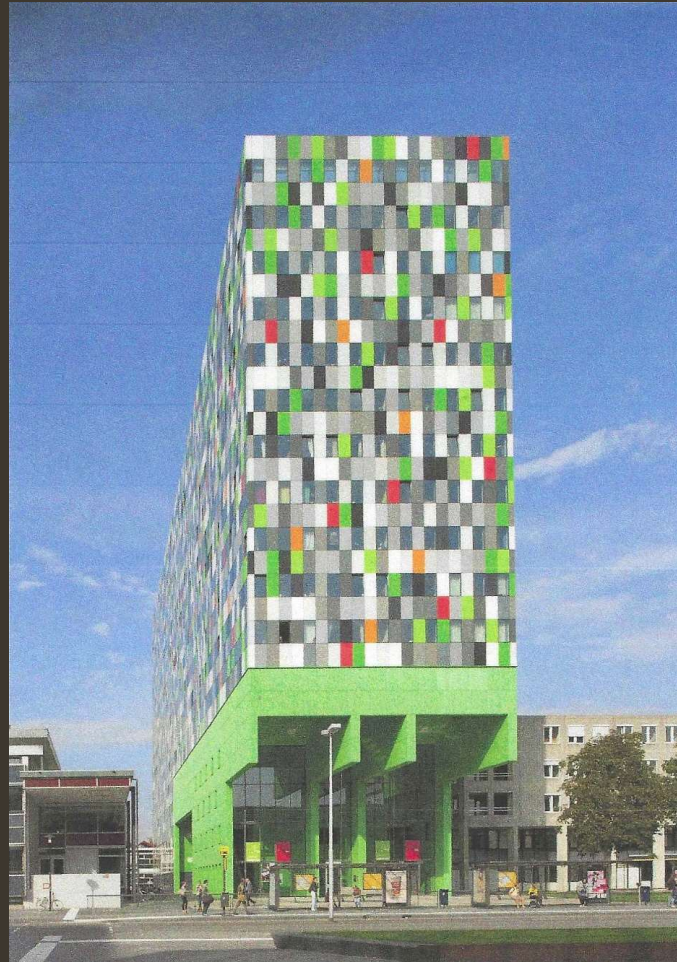
Hotel ceramic tile façade exterior concept
